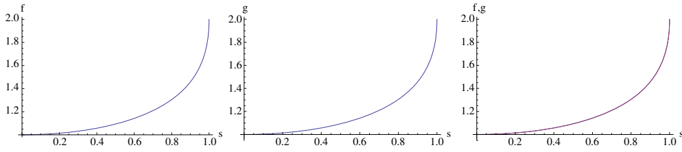
Figure 1. Graphics of f(\sigma) (left), g(\sigma) (center), f(\sigma) and g(\sigma) plotted together (right). In the figure, \sigma is labeled as s in the abscissa axis.
